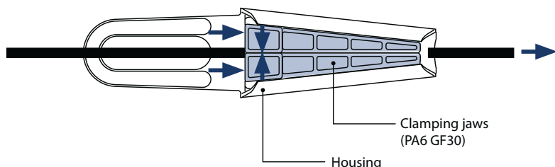
Clamping the cable under tensile stress
