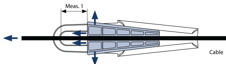
Open clamping jaws
